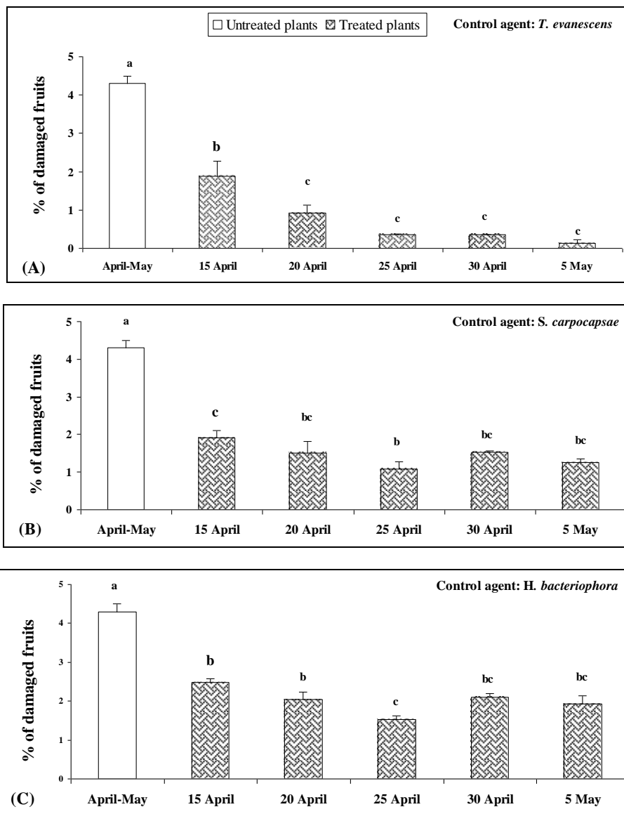
Fig. 1. Percentage of damaged (mean \pm SD) tomato fruits by H. zea larvae during various inspection dates of fruit maturation in treated plots by T. evanescens (A), S. carpocapsae (B) and H. bacteriophora (C) during 2005 growing season. Values superscripted by the same letter are not significantly different according to ANOVA, P < 0.05 (for A: F = 63.46 , d.f. = 5, 12; for B: F = 28.78 , d.f. = 5, 12; for C: F = 6.75 , d.f. = 5, 12).
