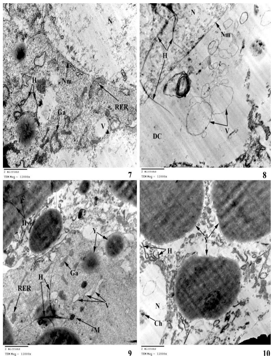
Fig.(4): 7-10 Electron micrograph of ovariols 7 -treated with mixture of M. anisopliae and neem 8 - treated with mixture of M. anisopliae and L-Glutamic acid. 9 - treated with mixture of M. anisopliae and S. molle . 10 -treated with with mixture of M. anisopliae and abamectin. basement membrane ( Bm ) destroyed cytoplasm ( DC ) chromatin ( Ch ) endoplasmic reticulum ( RER ) golgi apparatus ( Ga ) hypha ( H ) lipid droplets ( L ) mitochondria ( M ) nucleus ( N ) nucleus membrane ( Nm ) rupture in nucleus ( RN ) vasculization ( V )
